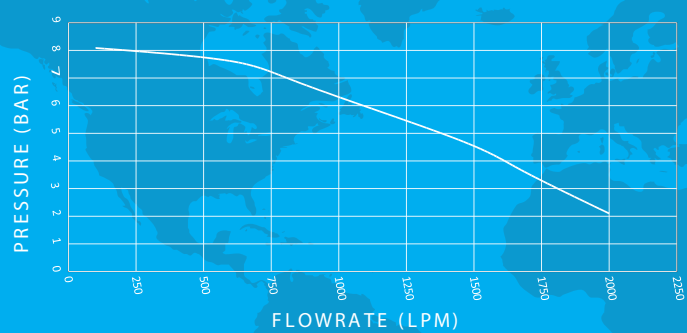
P2 GASOLINE MOTOPUMP PERFORMANCE CURVE
